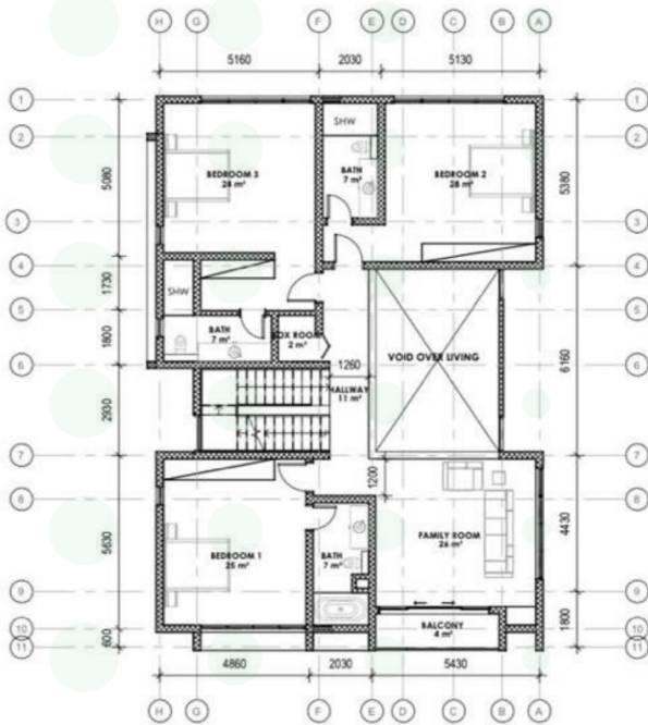
DETACHED- FIRST FLOOR PLAN 1:100
