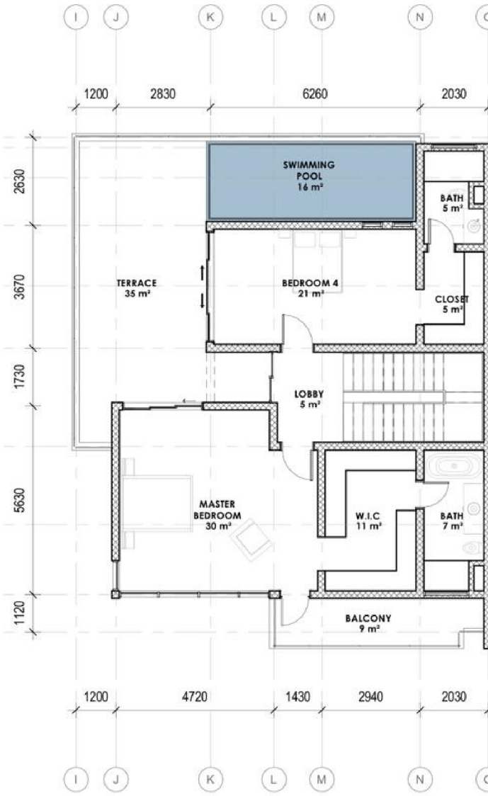
SEMI- SECOND FLOOR PLAN 1:100
