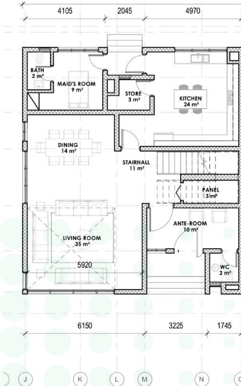
SEMI- GROUND FLOOR PLAN 1:100
