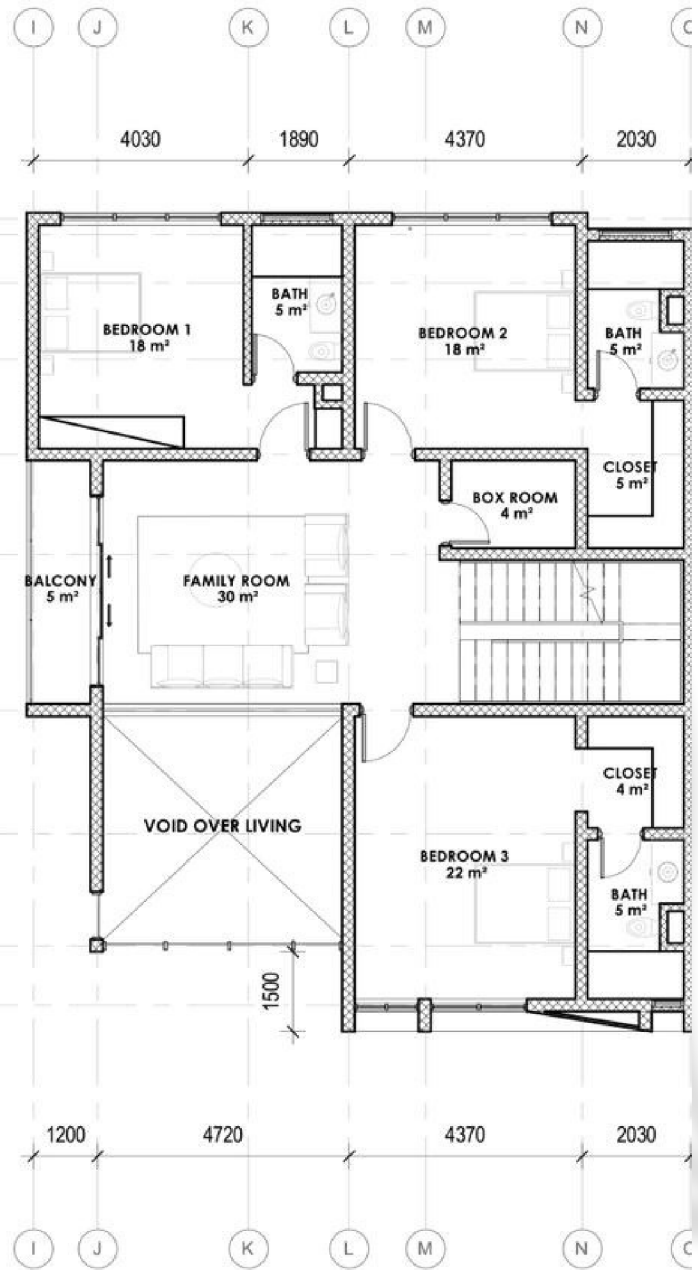
SEMI- FIRST FLOOR PLAN 1:100
