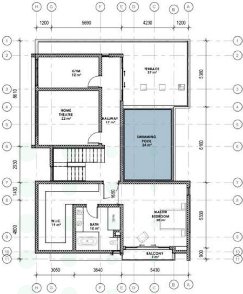
1 DETACHED- SECOND FLOOR PLAN 1:100
