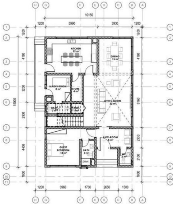
DETACHED- GROUND FLOOR PLAN 1:100
